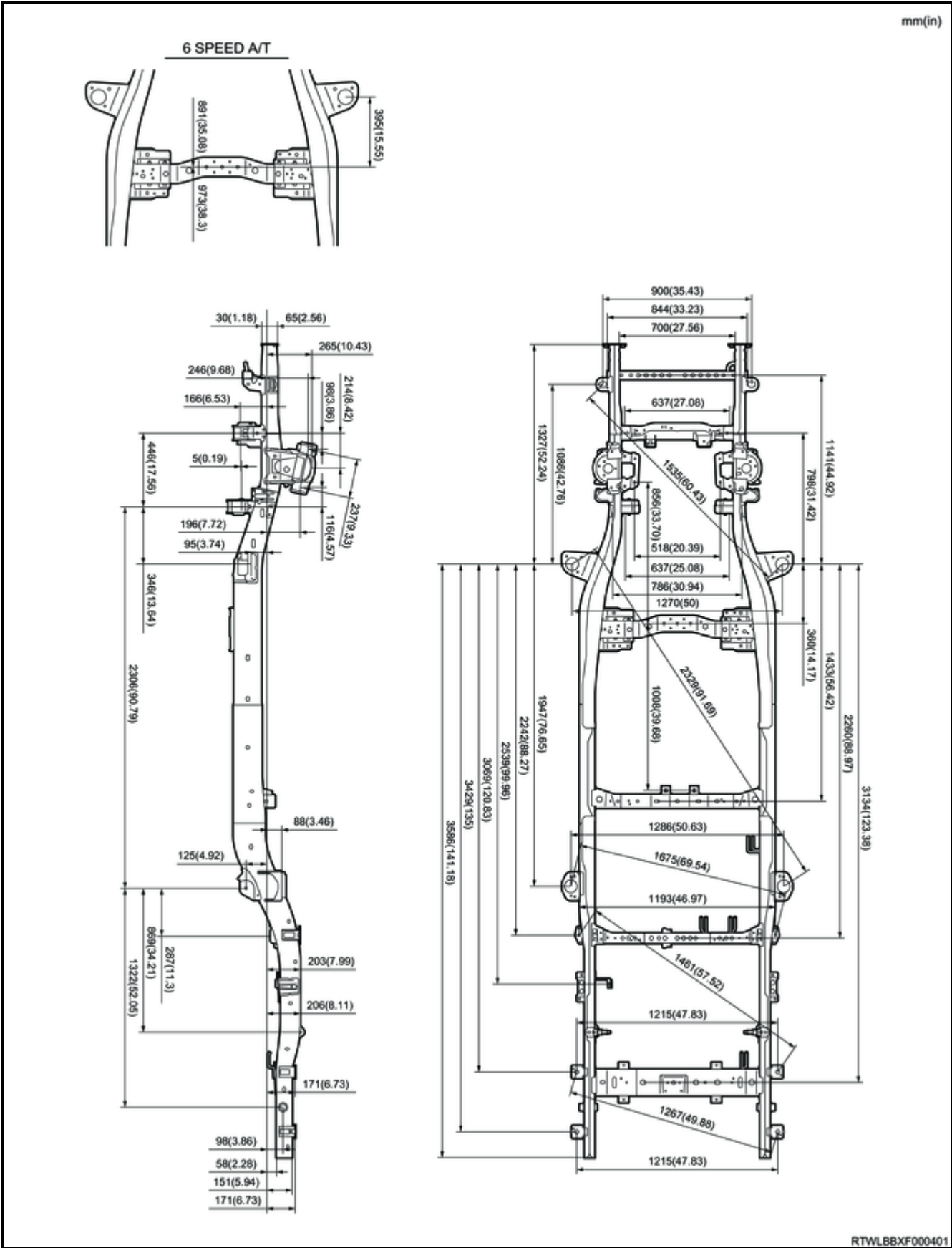
4WD (Standard cab)
