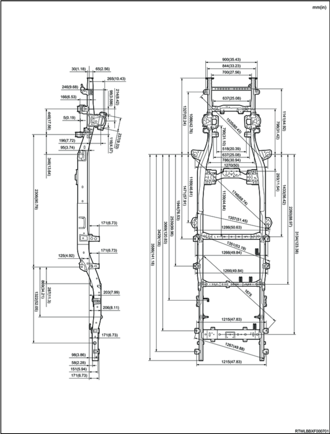
4WD (Extended cab)
